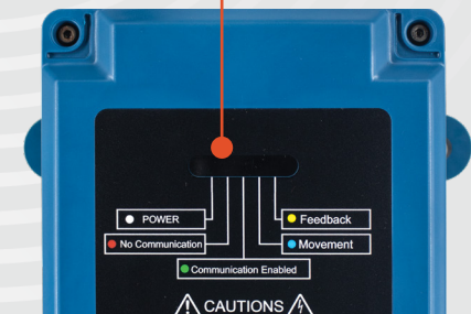
Feedback LED
