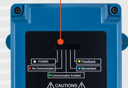
Feedback LED
